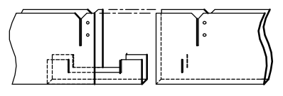
CONNECTION DETAIL
