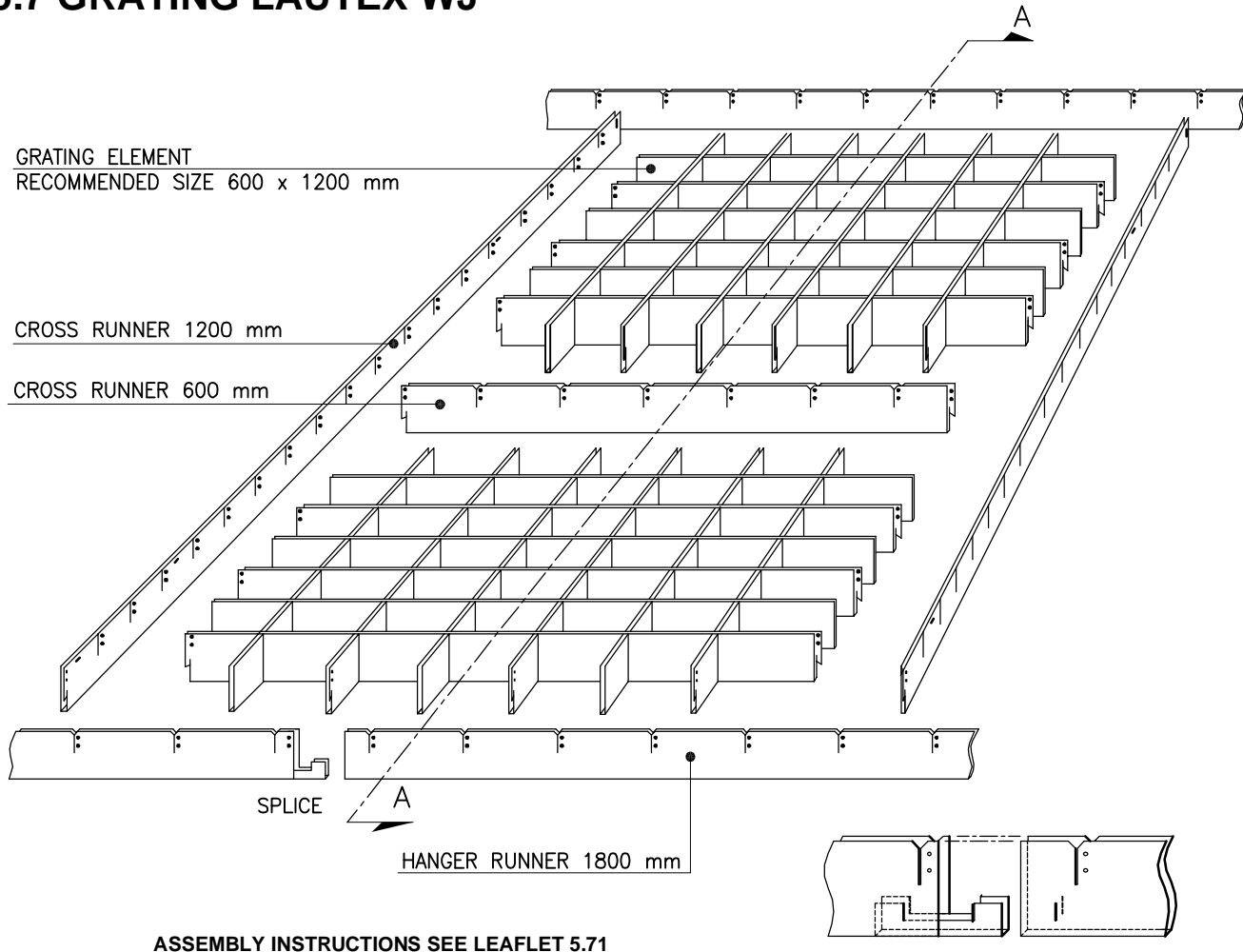
CONNECTION DETAIL
