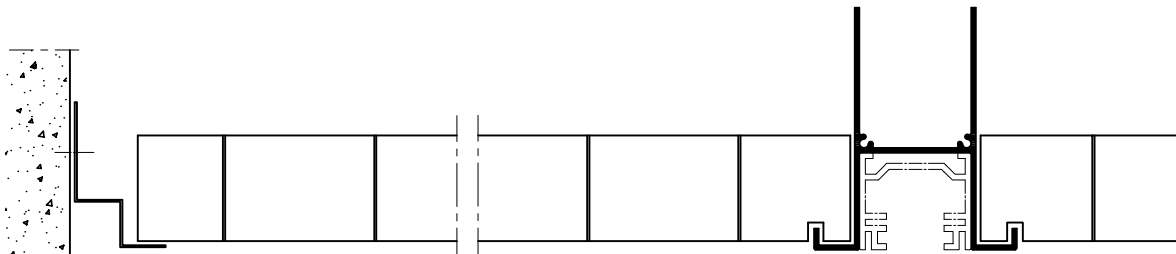
No. 14 DECORATIVE PROFILE KORISTEPROFIILI
